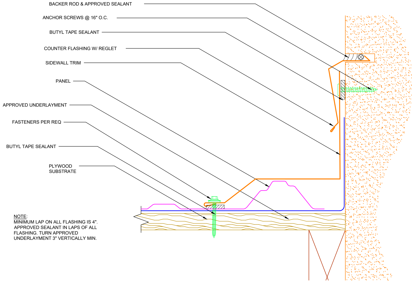
SW1 – Sidewall Detail
