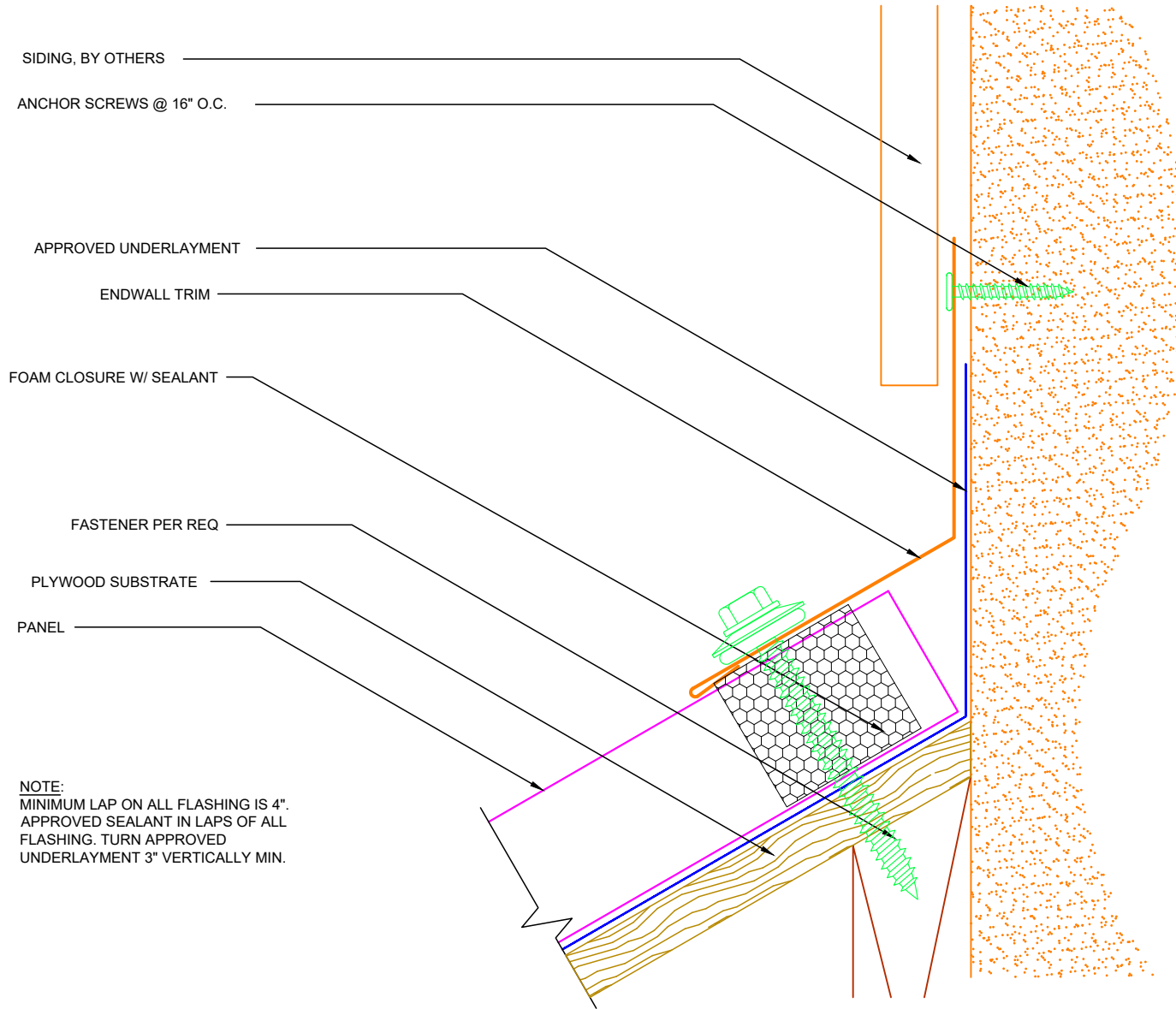
EW2 – Endwall Detail
