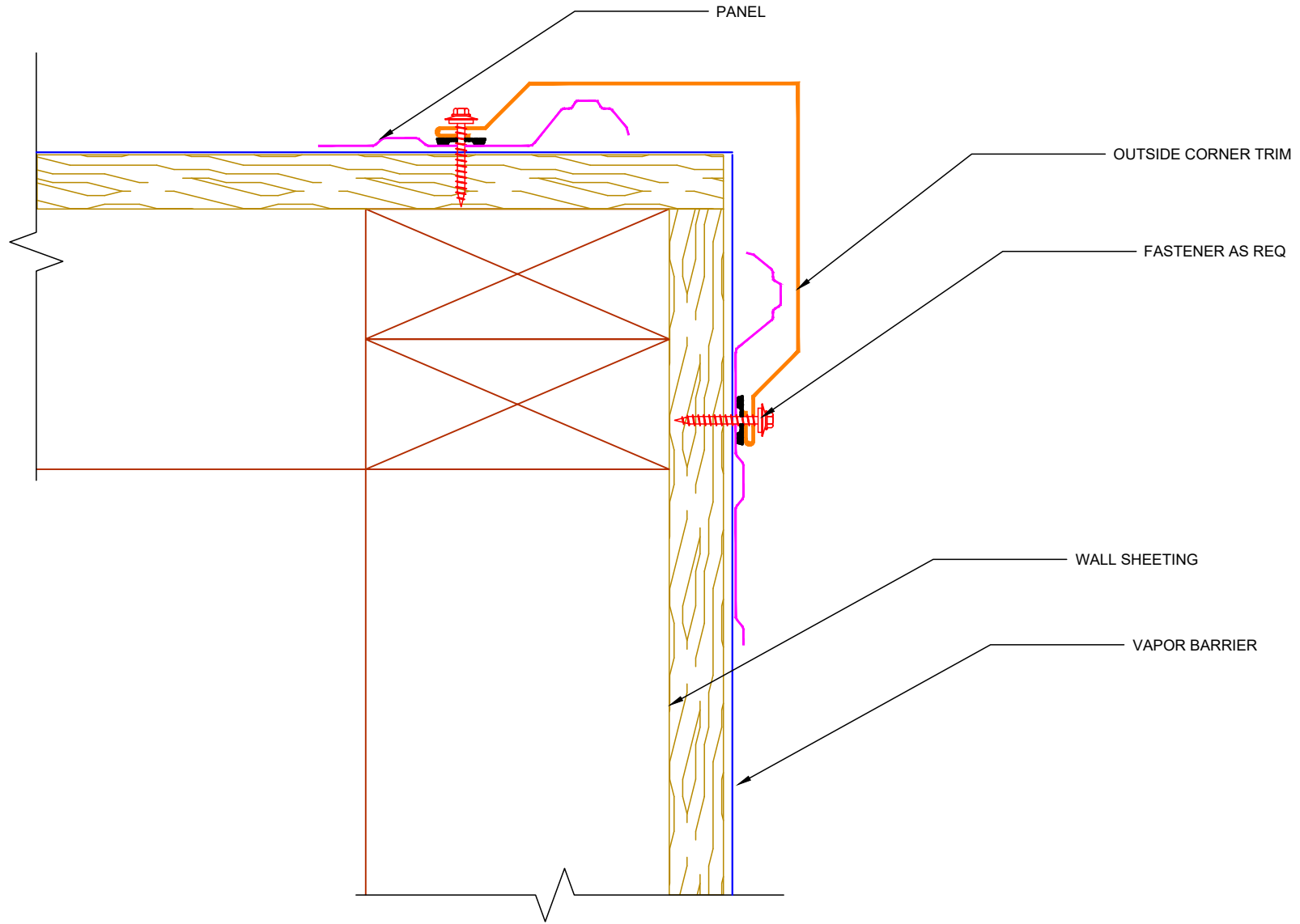
OSC – Outside Corner Detail
