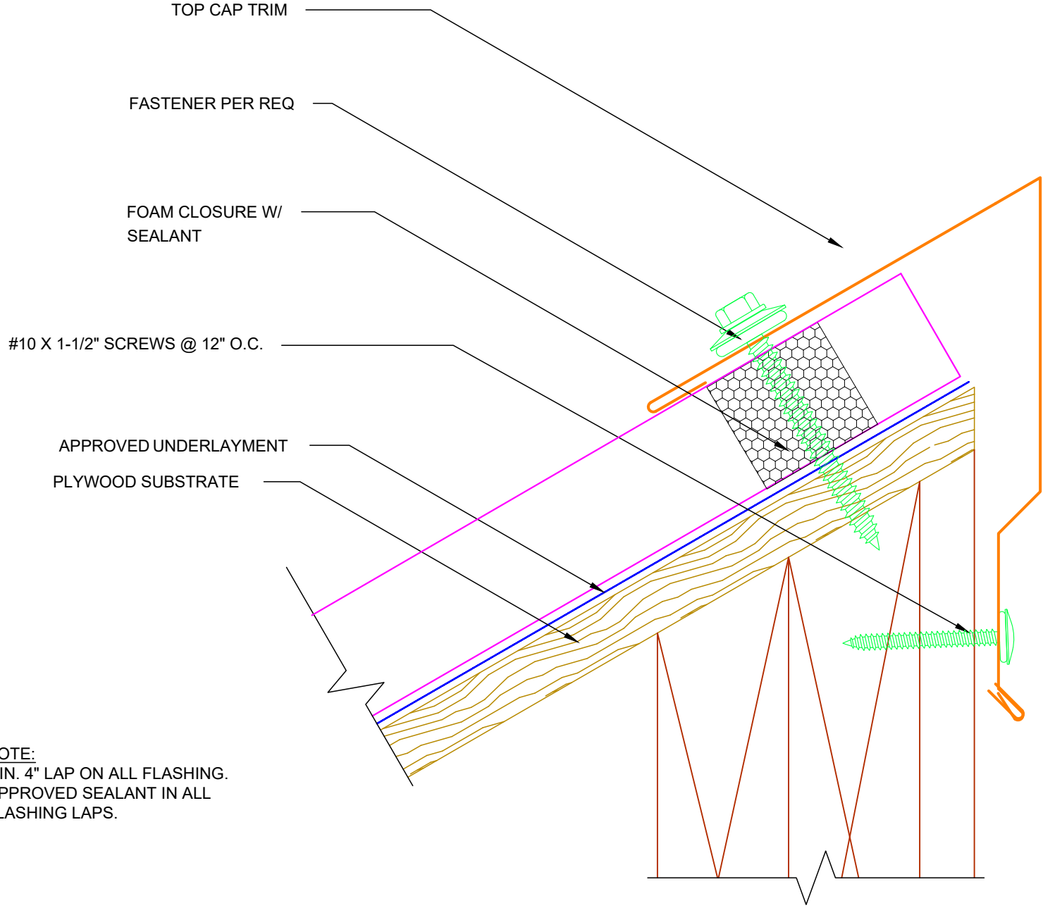
TC2 – 6" Top Cap Detail
